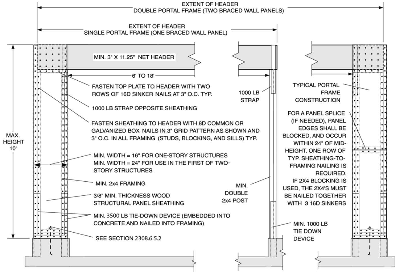
FIGURE 2308.6.5.2 PORTAL FRAME WITH HOLD-DOWNS (PFH)
