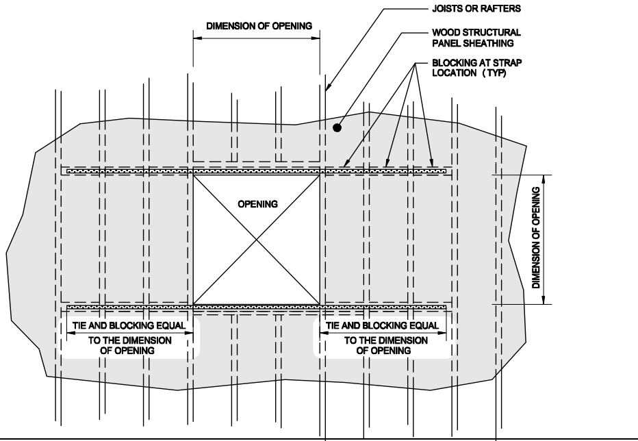
FIGURE 2308.4.4.1(1) OPENINGS IN FLOOR AND ROOF DIAPHRAGMS
